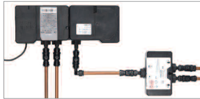
Processor connected to diverter with additional pipe
